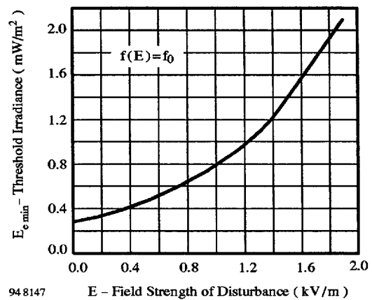
Figure 4 : Sensitivity vs. Electric Field Disturbances
