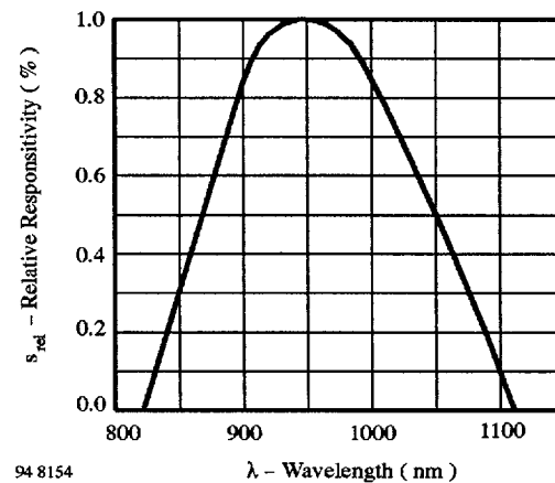
Figure 12 : Spectral Response
