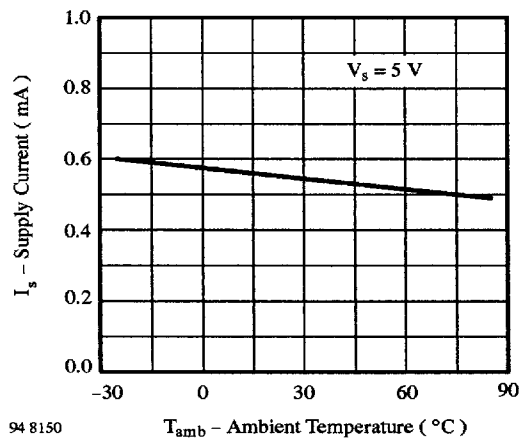
Figure 11 : Supply Current vs. Temperature
