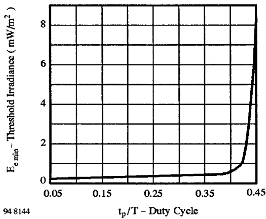
Figure 9 : Sensitivity vs. Duty Cycle
