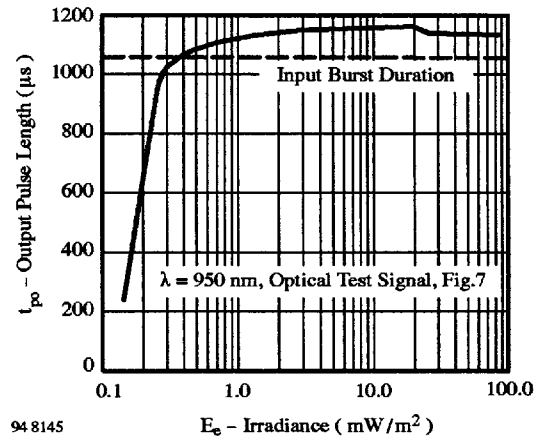
Figure 2 : Sensitivity in Dark Ambient
