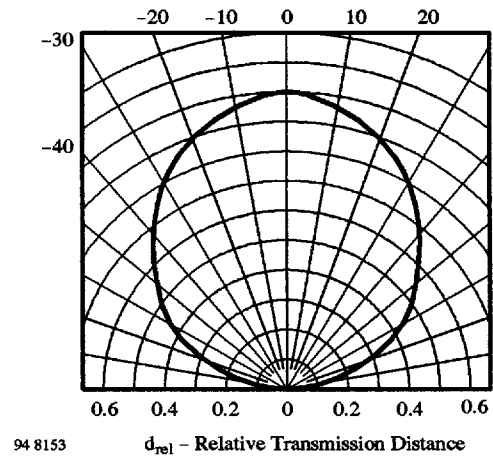
Figure 14 : Horizontal Directivity \phi_x
