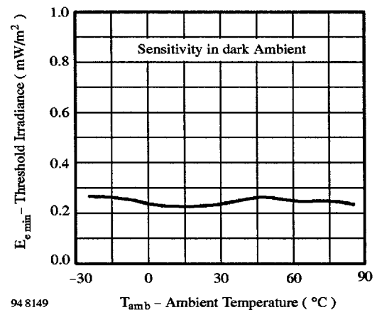
Figure 6 : Sensitivity vs. Temperature
